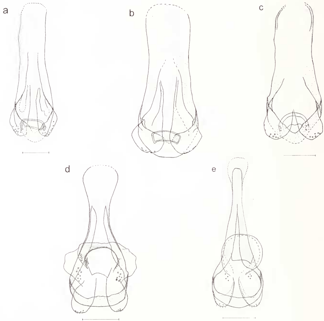
Fig. 6. Male genitalia a: Trochiloecetes rumpumuni , b: T. insularis , c: T. ochoterena , d: " Trochiliphagus ", e: Ricinus dolichocephalus (from RHEINWALD 1968, Fig. 13). Scale bar 0.1 mm.
